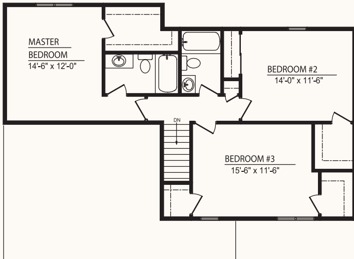
SECOND FLOOR PLAN (3) BEDROOM OPTION
