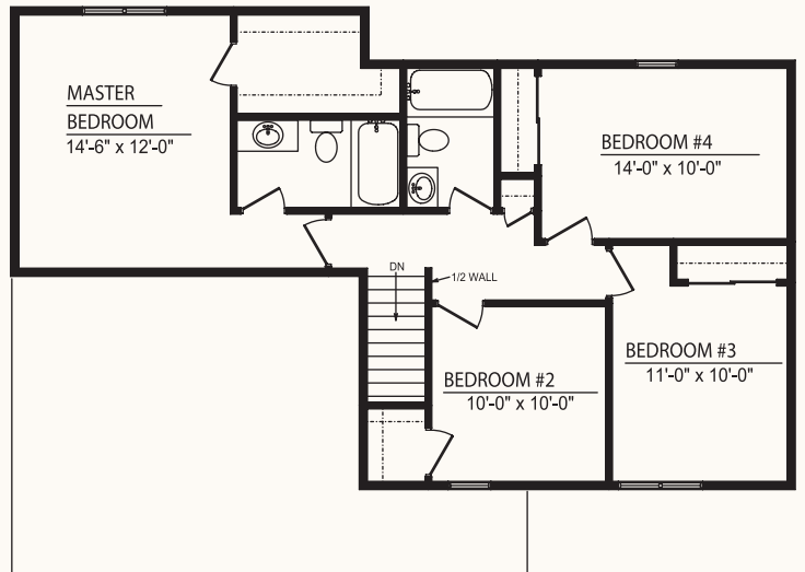
SECOND FLOOR PLAN (4) BEDROOM OPTION
