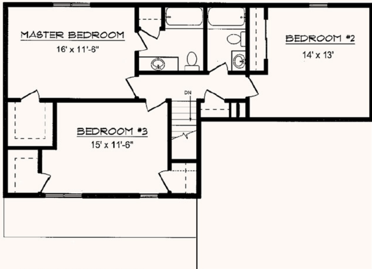
SECOND FLOOR PLAN (THREE BEDROOM OPTION) (FOUR BEDROOM OPTION AVAILABLE)
